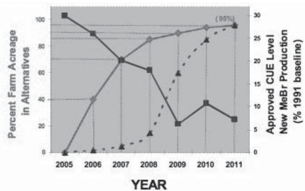
Figure 1. Statistical projection of forced rates of adoption of alternatives based on the CUE approved amounts of “new” methyl bromide production and consumption. The projection is based on assumptions of minimal “available Stocks”, 1991 use characteristics and 2005 base crop acreages.
